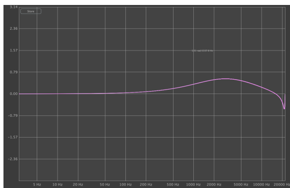
Phase response of a cramped EQ at 44.1kHz
