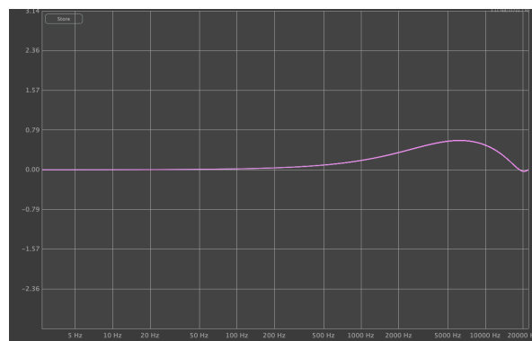
Phase response of de-cramped X-EQ 2 at 44.1kHz
