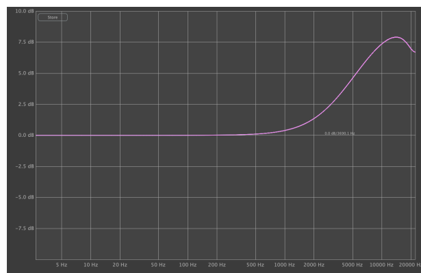
Frequency response of de-cramped X-EQ 2 at 44.1kHz
